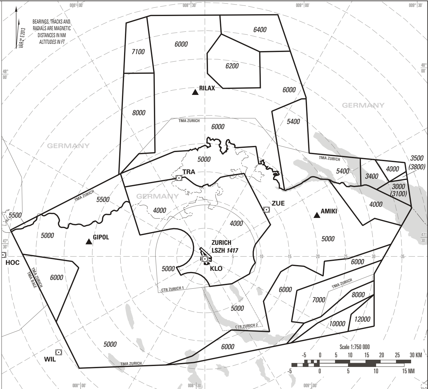
ATC SURVEILLANCE MINIMUM ALTITUDE CHART
