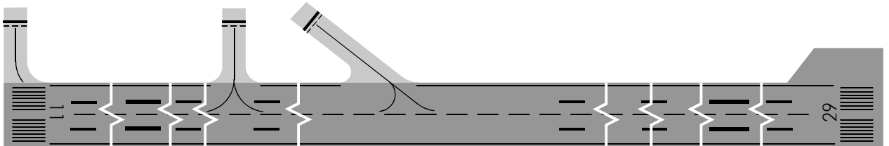
MARKING AIDS RWY 11 / 29 AND EXIT TWY
